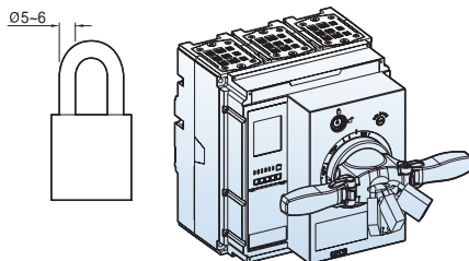
Locking at ON or OFF position
